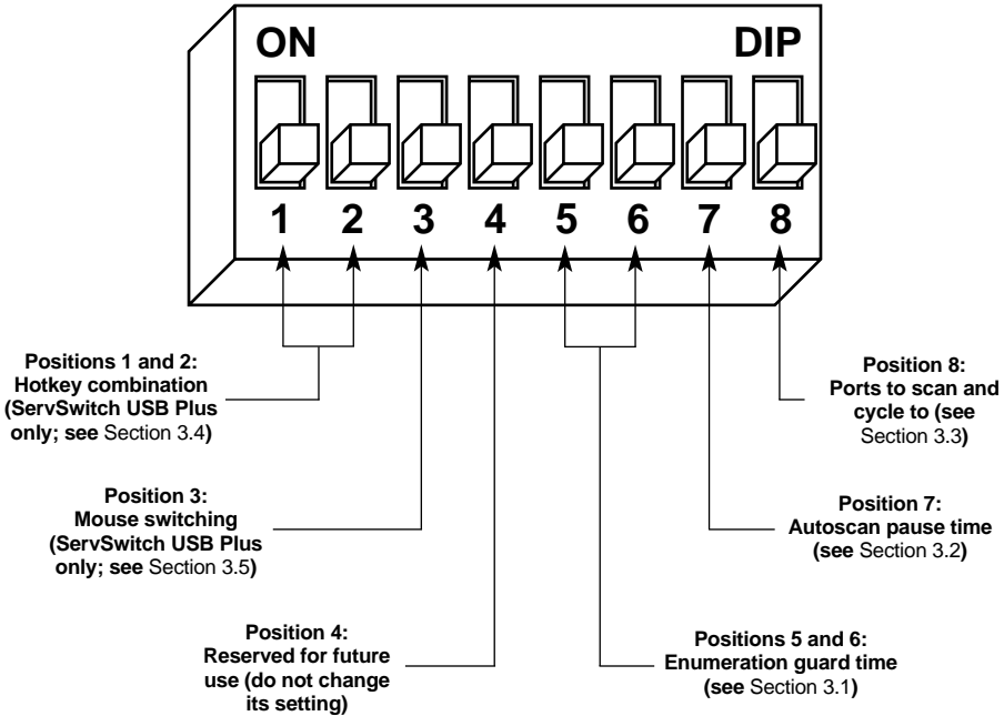
Figure 3-1. The configuration DIP switch.
